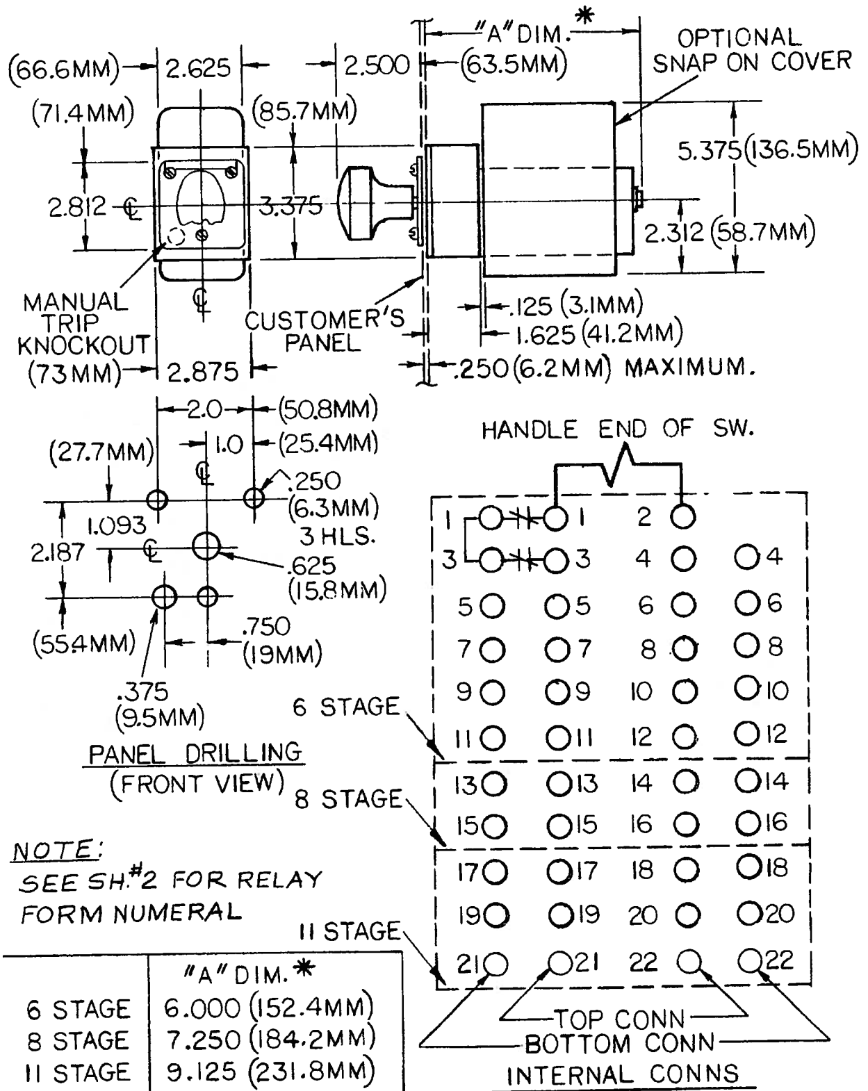
* Fig. 2 (0275A3211 Sh. 1 [3]) Outline, Panel Drilling and Internal Connections for Relay HSA11
